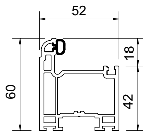
VS04 Standard Sash
